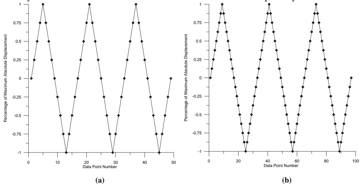
Figure 5: (a) Loading regime and data points for 0.25", 0.5" and 1" displacement levels; (b) all other displacement levels
